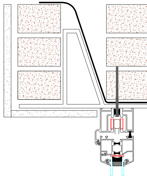
Catnic (with fixing screw fixed into the brick)
