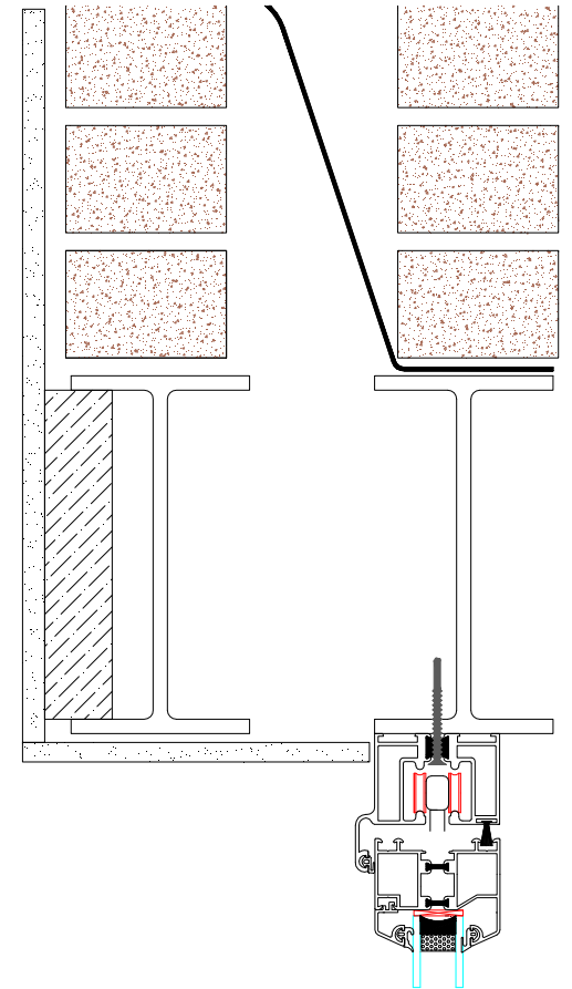
Re-enforced Steel Joist
