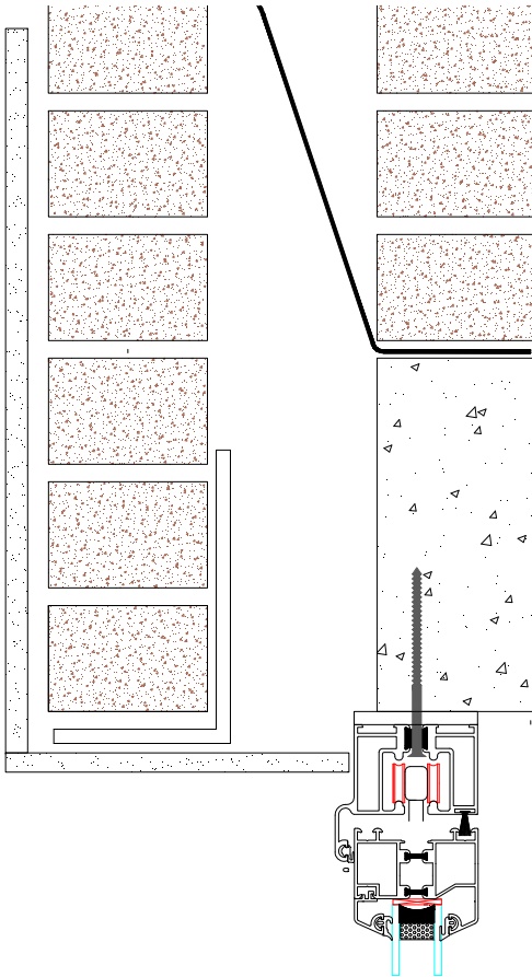
Concrete or Timber Lintel
